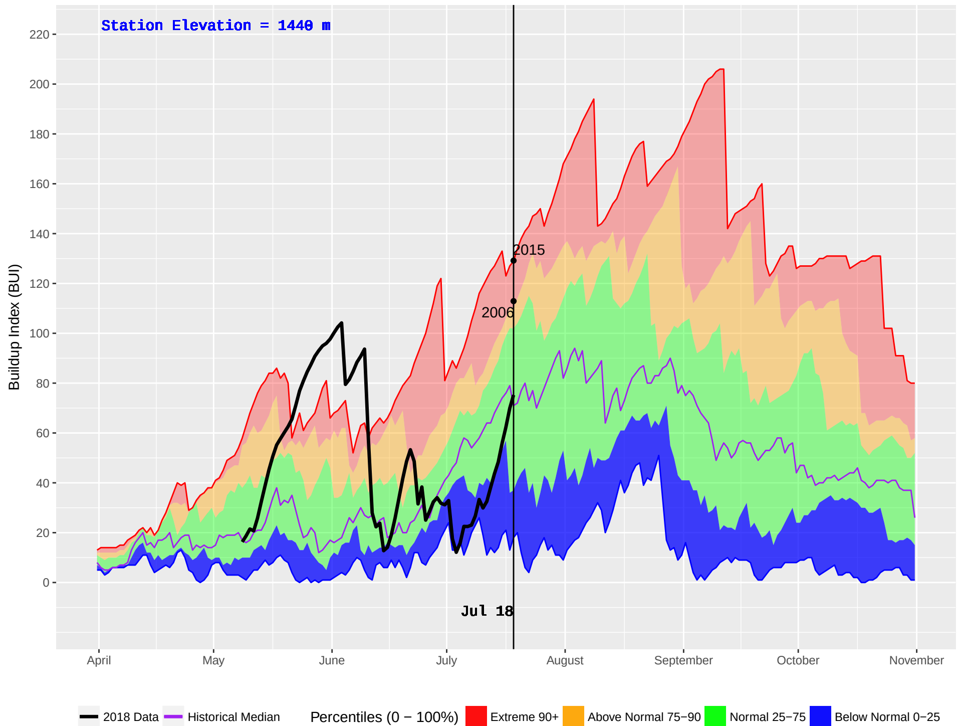
PASKA LAKE (326) : Historical (1999–2016) and Current (2018) Daily Buildup Index (BUI)
